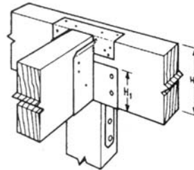
OPTION 2: CC + GLT
