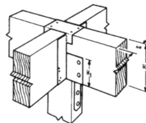
OPTION 1: CC + HWD (Saddle Hanger)
