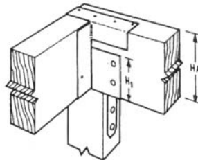
OPTION 1: ECC + HW (Offset Top Flange)
