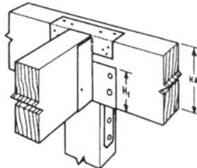
OPTION 1: CC + HW
