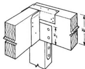
OPTION 2: ECC + GLT (Offset Top Flange)
