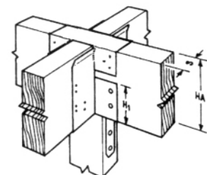
OPTION 2: CC + GLS (Saddle Hanger)
