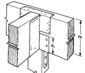
OPTION 3: CC + HGLT
