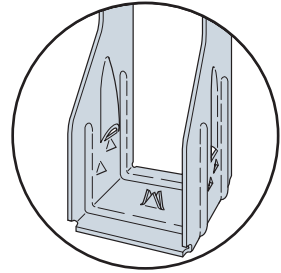
The Strong-Grip™ seat secures I-joists in position without joist nails
