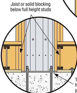
BALLOON FRAMING STACKED-WALL CONNECTION DETAIL
