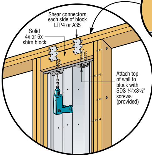
TOP-OF-WALL CONNECTION
