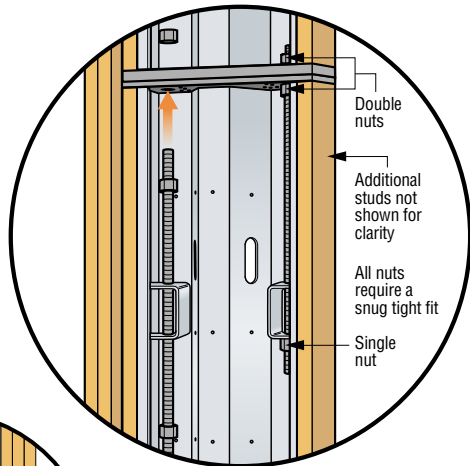
BALLOON FRAMING STACKED-WALL CONNECTION DETAIL
