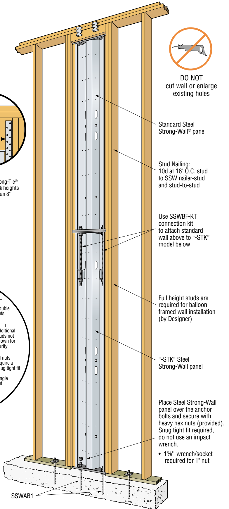
BALLOON FRAMING STACKED-WALL CONNECTION DETAIL
