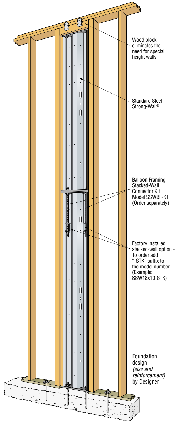
STACKED-WALL SOLUTION FOR BALLOON FRAMING
