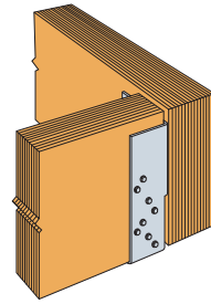
Typical MGU Installation with Right Flange Concealed
