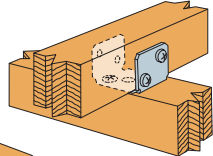
Typical RTU2 Installation (use SD8X1.25 screws, dry environments only)
