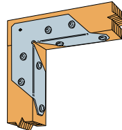
Typical RTA12 Installation (use SD8X1.25 screws, dry environments only)
