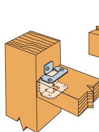
Typical RTR Installation (use SD8X1.25 screws, dry environments only)
