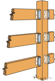
Typical FB26 Installation
