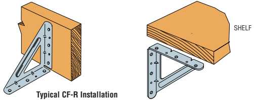
Typical CF-R Installation (use 10d commons or SDS \frac{1}{4} x2" screws)
