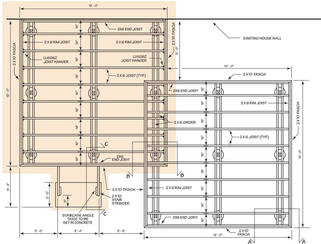
DECK FRAMING PLAN
