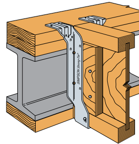
HIT Installation on a 3x Nailer mounted on a Steel Beam
