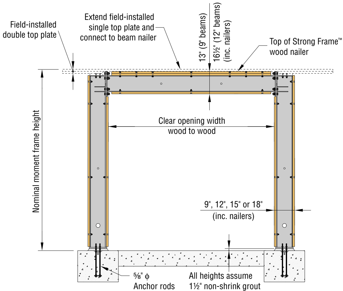
Assembly Elevation
