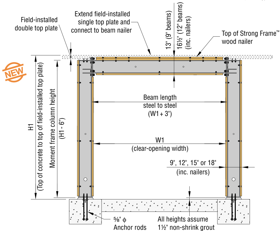
Assembly Elevation
