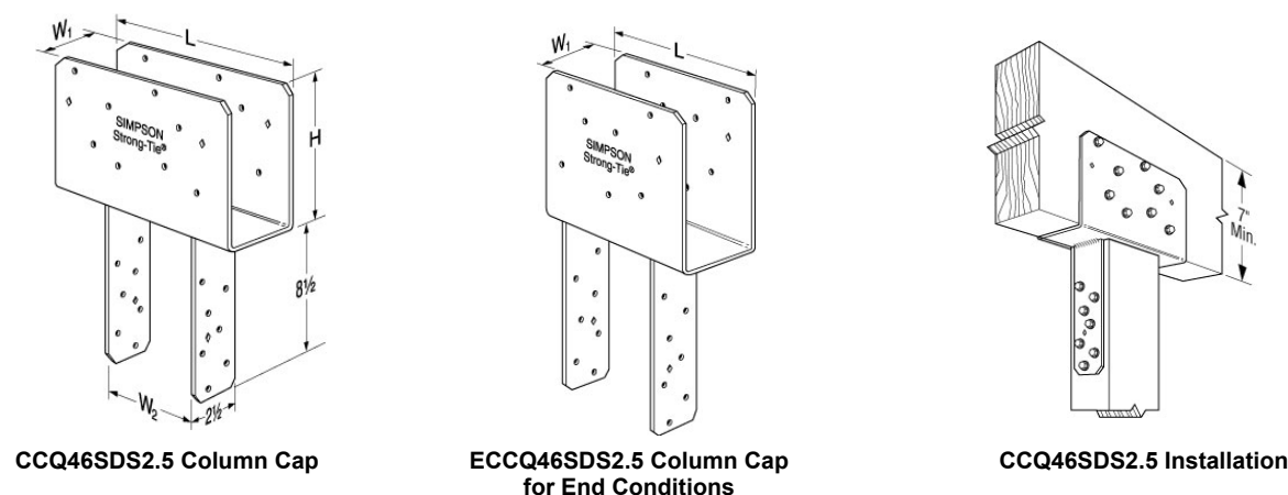
FIGURE 2—CCQ and ECCQ COLUMN CAPS
