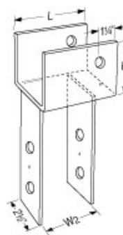
FIGURE 1—CC and ECC COLUMN CAPS
