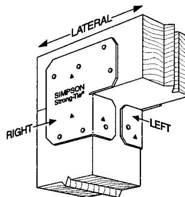
Figure 3b—Typical ACE Installation
