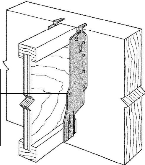
FIGURE 2—TYPICAL IUS INSTALLATION
