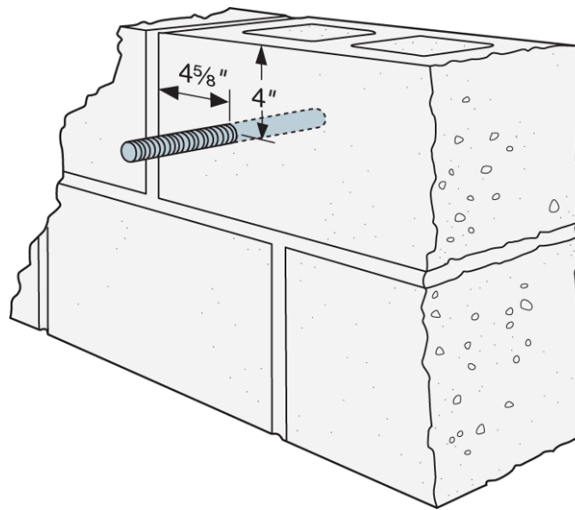
FIGURE 2—ANCHOR INSTALLATION IN HOLLOW CMU MASONRY WALL CONSTRUCTION [Minimum 4-inch (102 mm) Distance to Edge or End of Masonry Wall Construction and Minimum 4 5 / 8 -inch (117 mm) Distance to a Head Joint]
