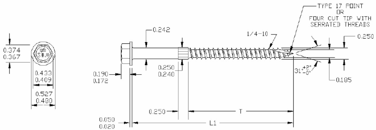
FIGURE 1—SDS SCREW
