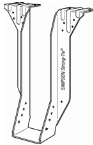
FIGURE 4a—BA SERIES HANGER
