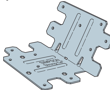
RBC - Bent 60° (Field bend one time only)
